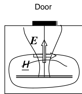
Field Pattern (Top View)
